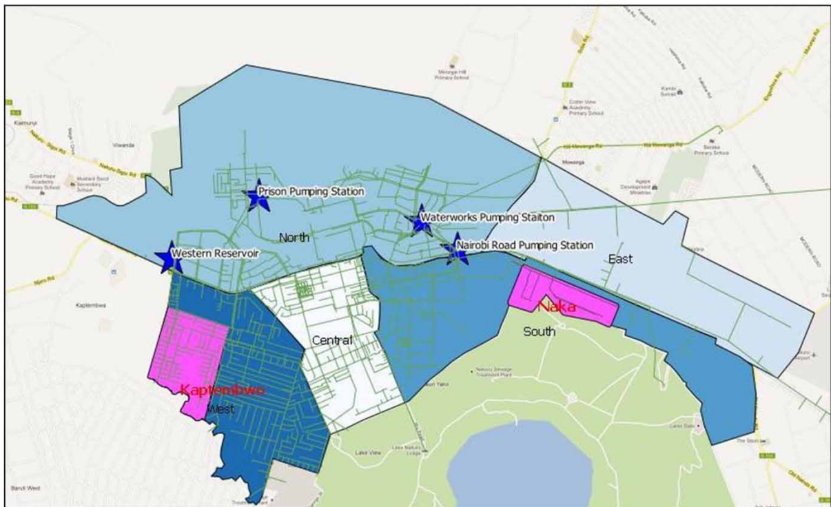
Map. 3. Location of zones/DMAs in NAWASSCO service area. A full colour version of this map is available online at http://www.iwaponline.com/wp/toc.htm .
