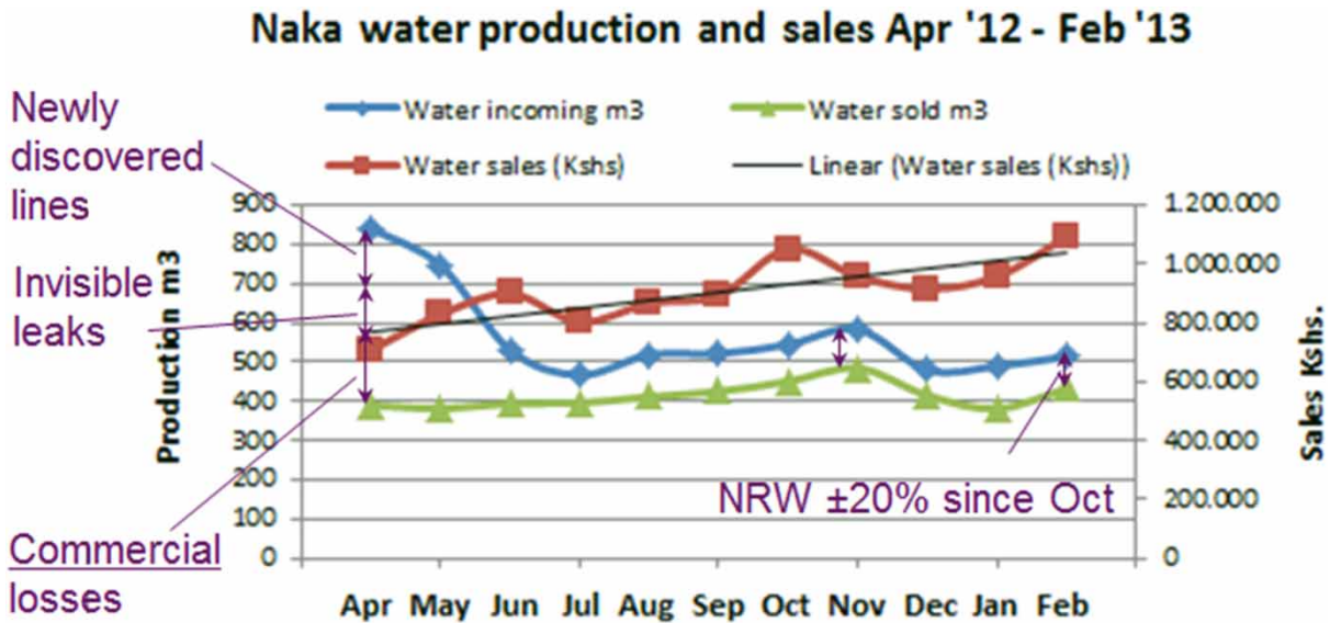
Fig. 13. NAKA water production and sales – April 2012 to February 2013.
