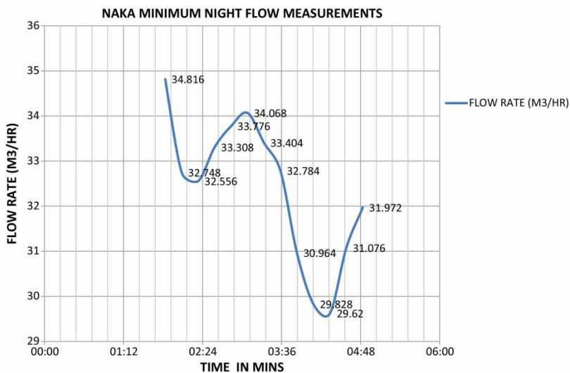
Fig. 6. Minimum night flow measurement results, NAKA.
