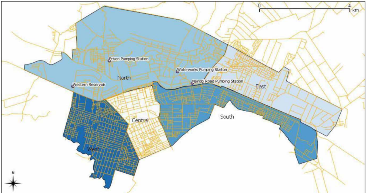
Map. 1. NAWASSCO's asset map with zones.
