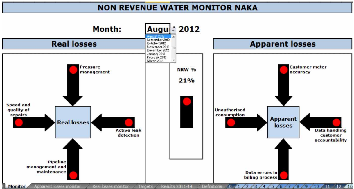
Fig. 8. The NRW monitor, NAKA.
